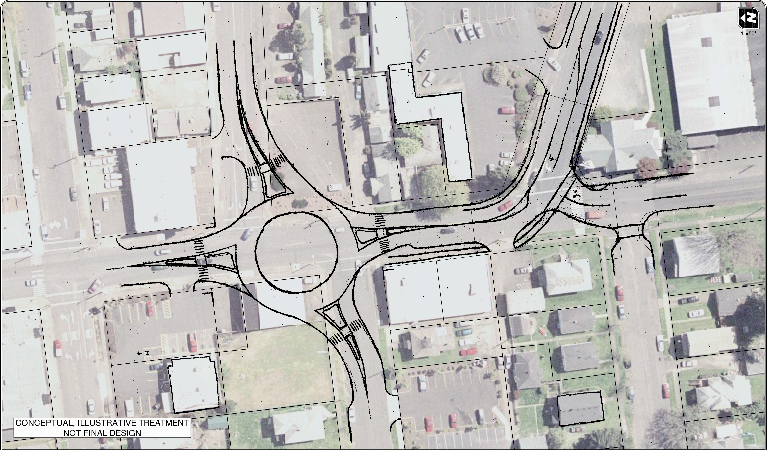
MAIN STREET/ SANTIAM ROAD/SALEM ROAD ALTERNATIVE ALBANY, OREGON
